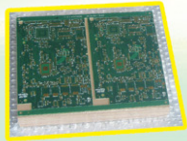
真空保護成品 VACUUM PACKAGED SAMPLES
